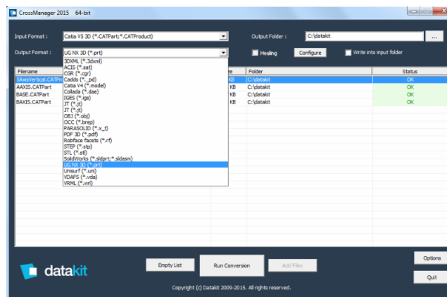
CrossManager Interface
